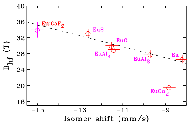
Fig. 1 Plot of hyperfine field ( B_{\text{hf}} ) vs. isomer shift ( \delta ) for a variety of \text{Eu}^{2+} compounds taken from the compilation by Wickman et al. [18]. The dashed line is a linear fit (omitting \text{EuCu}_2 ) with a slope of -1.4(3) T/(mm/s)
