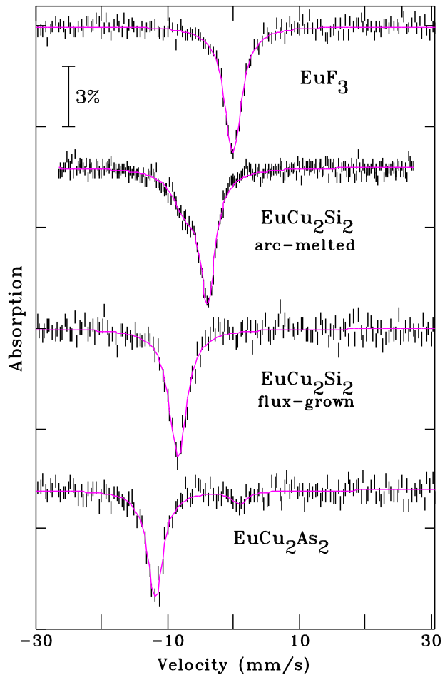
Fig. 2 Some typical ambient temperature paramagnetic ^{151}\text{Eu} Mössbauer spectra showing the progression of isomer shifts. \text{Eu}^{3+} in \text{EuF}_3 has an isomer shift close to zero. Arc-melted \text{EuCu}_2\text{Si}_2 is intervalent with two components evident, both of which show more negative shifts than \text{EuF}_3 , while flux-grown single-crystal \text{EuCu}_2\text{Si}_2 is fully divalent. \text{EuCu}_2\text{As}_2 exhibits a close to extremal isomer shift for divalent intermetallic compounds. The additional feature near 0 mm/s is due to \text{Eu}_2\text{O}_3
