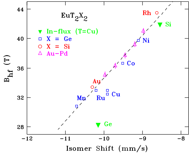
Fig. 4 Hyperfine fields ( B_{\text{hf}} ) vs. isomer shifts for a variety of \text{EuT}_2\text{X}_2 compounds. Most of the open symbols are taken from the compilation by Grandjean and Long [16], except for those labelled “Au–Pd” which are taken from work on \text{Eu}(\text{Pd}_{1-x}\text{Au}_x)_2\text{Si}_2 [42]. The solid symbols are taken from our (unpublished) work. The dashed line is a fit and has a slope of +5.8(4) T/(mm/s)
