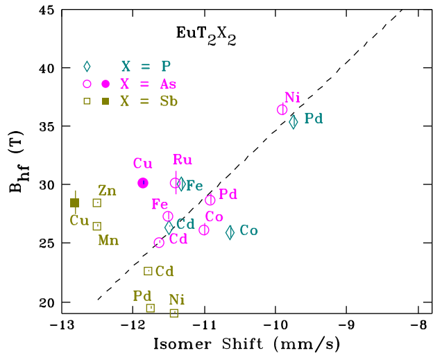
Fig. 5 Hyperfine fields ( B_{\text{hf}} ) vs. isomer shifts for a variety of \text{EuT}_2\text{X}_2 compounds where X is a pnictide (P, As, Sb). Phosphides: Cd [45], Co [46, 47], Fe [46, 48, 49], Pd [50]; Arsenides: Cd [45], Co [43], Fe [51], Ni [43], Pd [43], Ru [52]; Antimonides Cd [45], Mn [53], Ni [54], Pd [55], Zn [53]. The solid symbols are taken from our own (unpublished) work. The dashed line is the same fit as used in Fig. 4 and is included for context
