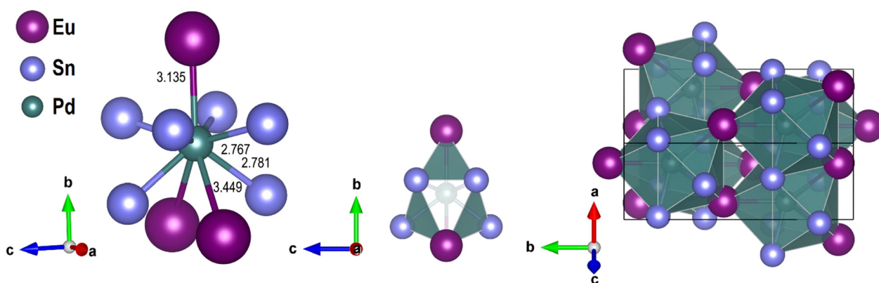
Fig. 1 On the left: The coordination around the central Pd atom (bond distances in Å). At the center: The basic tricapped trigonal prism of composition [ \text{PdEu}_3\text{Sn}_6 ] centred by Pd and viewed along the main axis. On the right: Overall crystal structure of \text{EuPdSn}_2 showing an extended unit cell.
