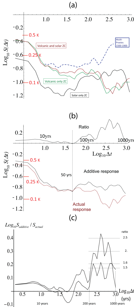
Figure 3. (a) The RMS Haar fluctuations of the Zebiak–Cane (ZC) model responses (from an ensemble of 100 realizations) with volcanic only (green, from the updated Crowley reconstruction), solar only (black, using the sunspot-based background; Wang et al., 2005), and both (brown). No anthropogenic effects were modelled. Also shown for reference are the fluctuations for three multiproxy series (blue, dashed, from 1500 to 1900, pre-industrial; the fluctuations statistics from the three series were averaged, and this curve was taken from Lovejoy and Schertzer, 2012b). We see that the combined volcanic and solar response of the model reproduces the statistics until scales of \approx 50 –100 years; however, at longer timescales, the model fluctuations are much too weak – roughly 0.1 K (corresponding to \pm 0.05 K) and constant or falling – whereas at 400-year scales, the temperature fluctuations are \approx 0.25 K ( \pm 0.125 ) and rising. (b) A comparison of the RMS fluctuations of the ZC model response to combined solar and volcanic forcings (brown, bottom, from a), with the theoretical additive responses (black, bottom) as well as their ratio ( S_{\text{additive}}/S_{\text{actual}} black, top). The additive response was determined from the RMS of the solar-only and volcanic-only response variances (from a): additivity implies that the fluctuation variances add (assuming that the solar and volcanic forcings are statistically independent). We can see that, after about 50–200 years, there are strong negative feedbacks, and the solar and volcanic forcings are subadditive; see (c) for an enlargement of the ratio. (c) An enlarged view of the ratio of the linear to nonlinear responses (from b). The top curve assumes for the combined forcing, the linearity of the response and statistical independence of the solar and volcanic forcings, whereas the bottom curve uses the actual response to the combined forcings. The maximum at around 400 years (top curve) corresponds to a factor \approx 2 ( \approx 1.5 , bottom curve) of negative feedback between the solar and volcanic forcings. The decline at longer durations ( \Delta t 's) – especially the single 1000-year fluctuation – is likely to be an artefact of the limited statistics at these scales.
