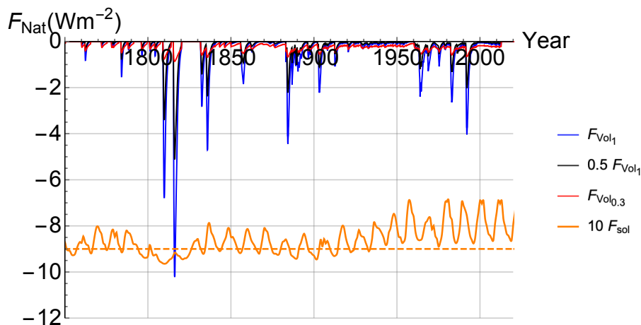
Figure 2. Volcanic forcing F_{Vol_1} (blue) is shown alongside two non-linearly transformed versions. Linearly damped by a constant 0.5 coefficient (black), and non-linearly transformed using equation with \nu = 0.3 (red). The solar forcing F_{Sol} (orange) has been shifted down by -9 and amplified by a factor of 10 for clarity. Adapted from (Hébert et al., 2020)
