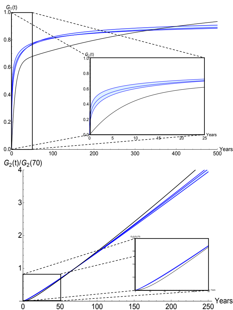
Figure 6. (top) The median and 90% CI of the FEBE step-response Green's function, G_1(H, \tau; t) , compared to the IPCC two-box model Green's function (black). (bottom) The median and 90% CI of the FEBE normalized ramp-response Green's function, G_2(H, \tau; t) , compared to the IPCC two-box model Green's function (black).
