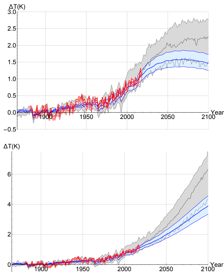
Figure 11. The forced temperature response projected using the FEBE, with parameters calibrated using F_{AerSSP} (blue), compared with the CMIP6 projection (black); 90% CI are indicated (shaded). The projections until 2100, for SSP 126 (top), and SSP 585 (bottom), are shown.
