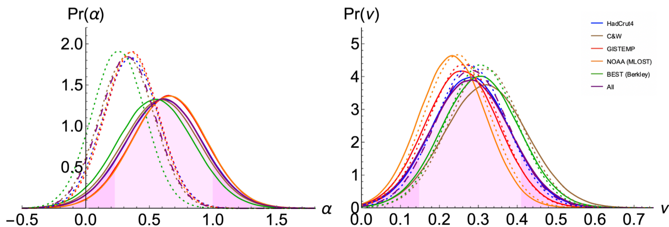
Figure 4. For each observational dataset and their average, PDFs are shown for the forcing parameters: the aerosol scaling factor \alpha (left), and the volcanic intermittency correction exponent \nu (right). Again, shown are the PDFs for parameter estimation based on both F_{Aer_{RCP}} (solid) and F_{Aer_{SSP}} (dashed). The average PDFs of the five observation datasets using F_{Aer_{RCP}} is shown as the main result with shading, with darker 5% tails
