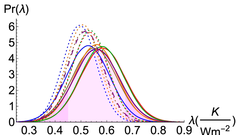
Figure 7. For each observational dataset and their average, PDFs are shown for the climate sensitivity parameter \lambda (the ECS, here in units of K(Wm^{-2})^{-1} ), F_{Aer_{RCP}} (solid) and F_{Aer_{SSP}} (dashed)
