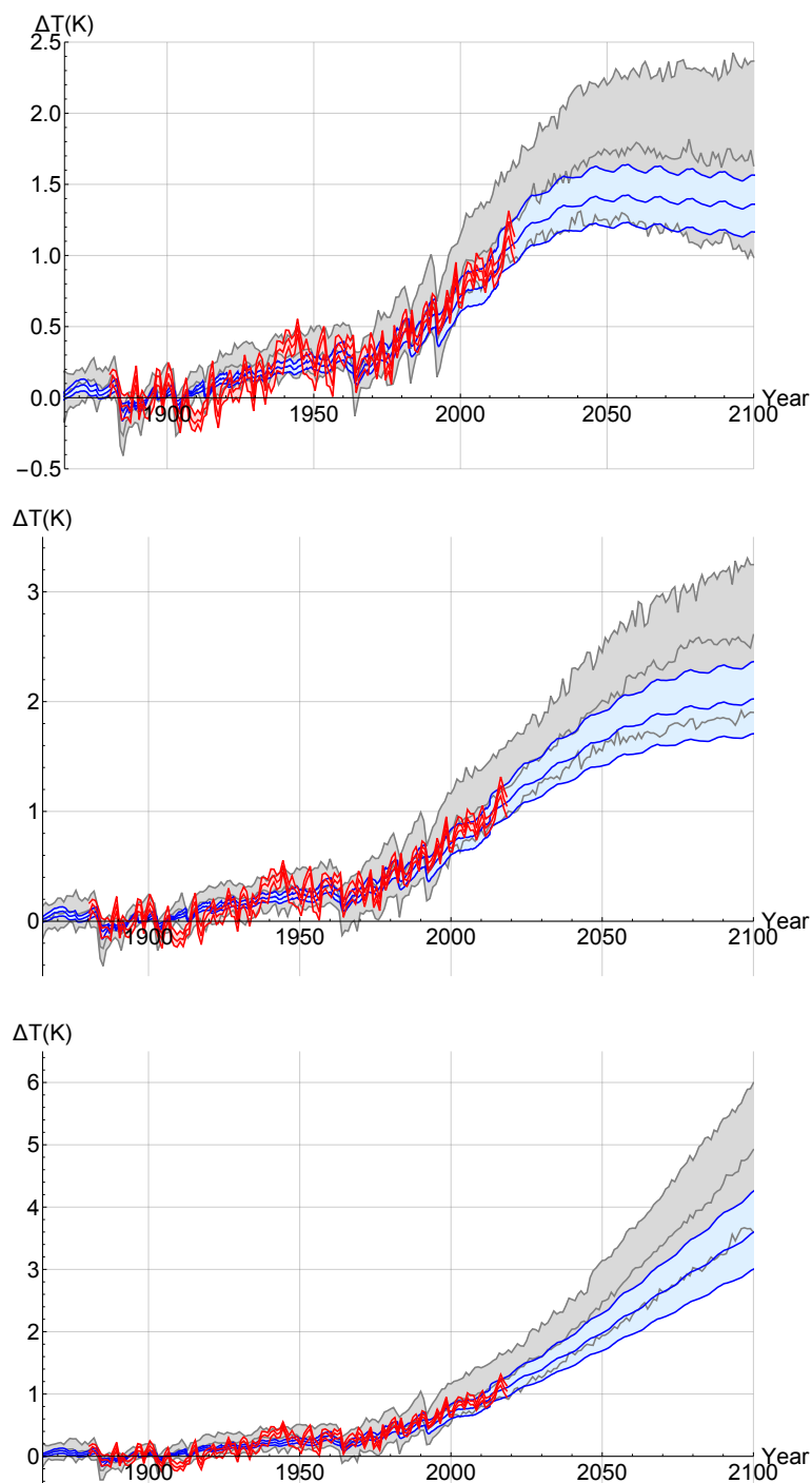
Figure 10. The forced temperature response projected using the FEBE, with parameters calibrated using F_{AerRCP} (blue) compared with the CMIP5 MME projection (black); 90% CI are indicated (shaded). The projections until 2100, for RCP 2.6 (top), RCP 4.5 (middle) and RCP 8.5 (bottom), are shown.
